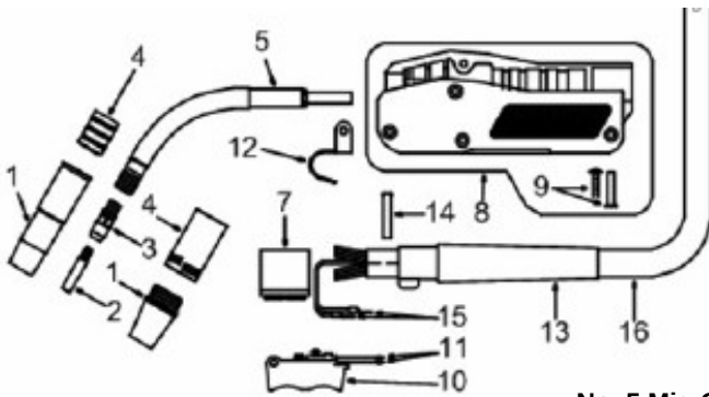
No. 5 Mig Guns
